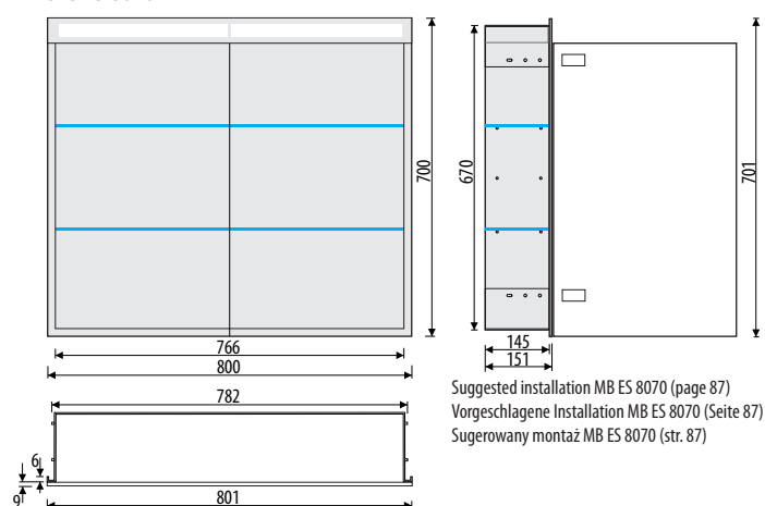
SPS ES 8070 LED
