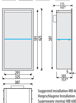
B.PWNP 3070/10 LED B.PWNP 3070/15 LED*
