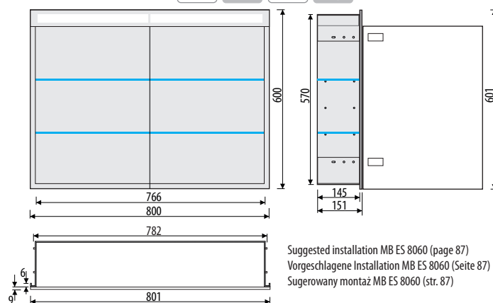
SPS ES 8060 LED
