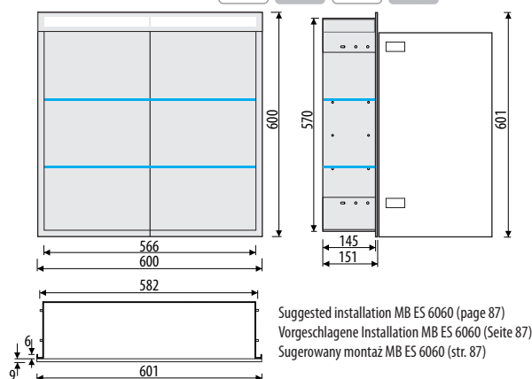
SPS ES 6060 LED
