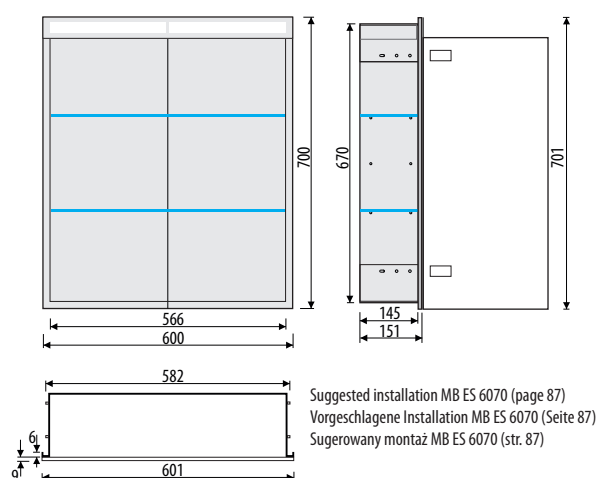
SPS ES 6070 LED
