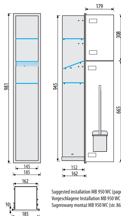
Z.PW2D LBL WC 950
